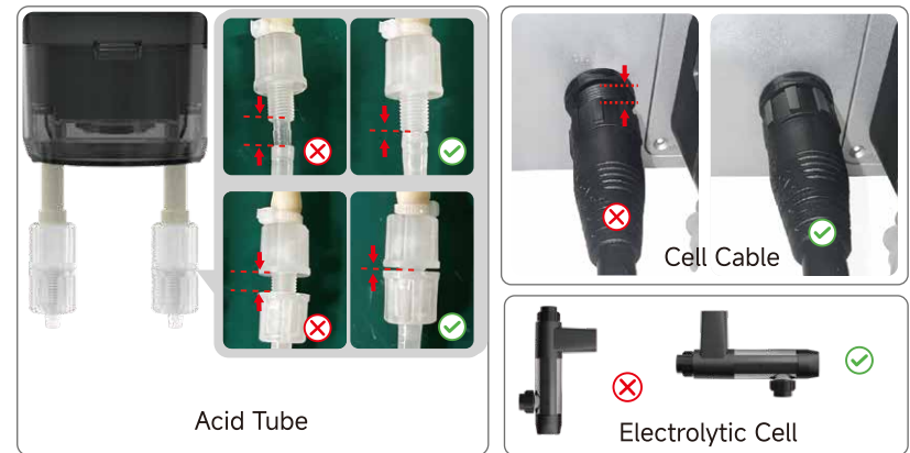
④ Probe & Connection Detail
