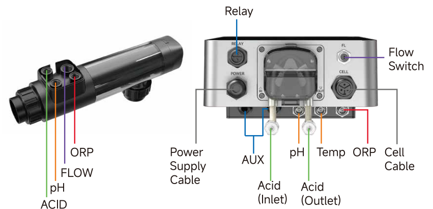
④ Probe & Connection Detail
